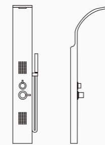
RL-P217B 1455*200*70mm Top Part 450mm
