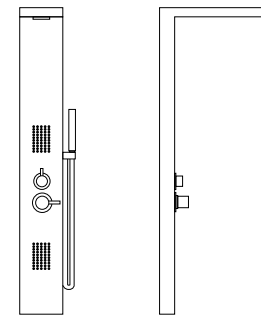
RL-P219B 1420*203*70mm Top Part 506mm
