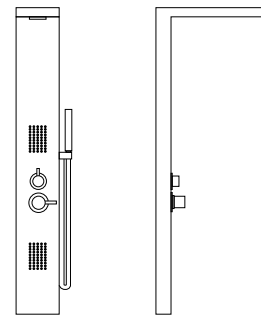
RL-P219W 1420*203*70mm Top Part 506mm
