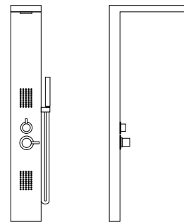
RL-P219 1420*203*70mm Top Part 506mm
